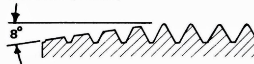
BOTTOMING No. 3 (2 THREADS)
